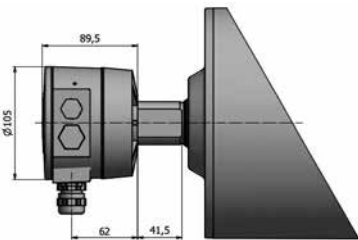
Large terminal Box \geq 5,5 kW
