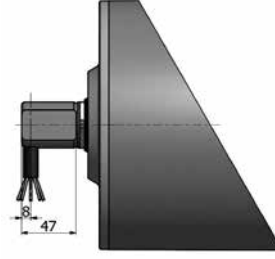
Cable slot 90° with threaded shaft
