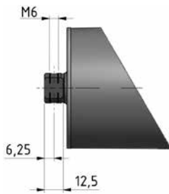
Cross-drilled and threaded shaft
