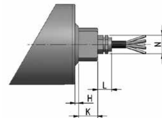
Straight connector
