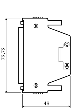
A6CON2
