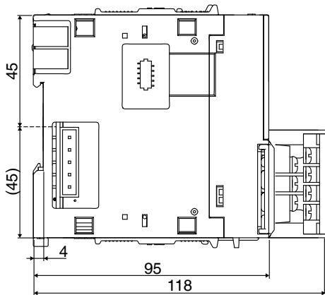
L26CPU-BT, L26CPU-PBT
