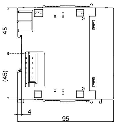
L02SCPU, L02SCPU-P
