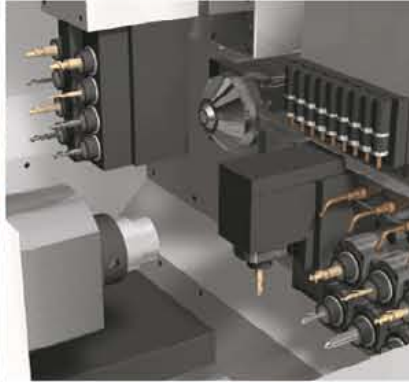
Automatic lathe
